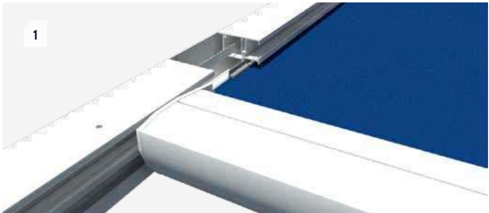
Thanks to the ZIP-screen technology the fabric is kept secure in the guide.
